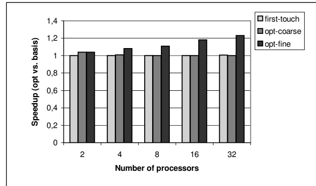
Figure 3. Improvement in execution time with the LU application
