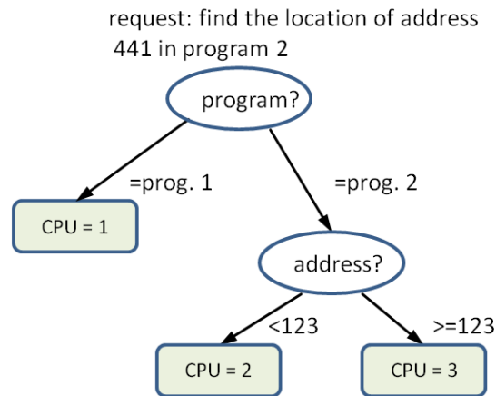
Figure 1. A sample decision tree for predicting a processor node
