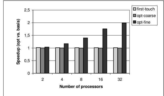
Figure 6. Improvement in execution time with the RADIX application
