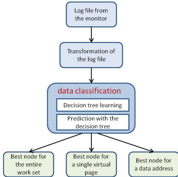
Figure 2. The analysis procedure for processing performance data
