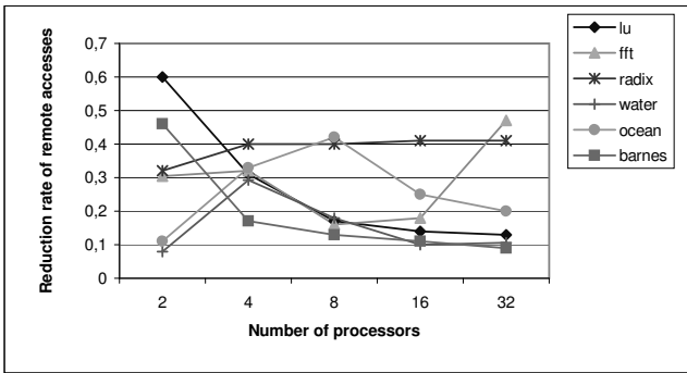
Figure 5. Reduction rate of remote accesses on different system scales
