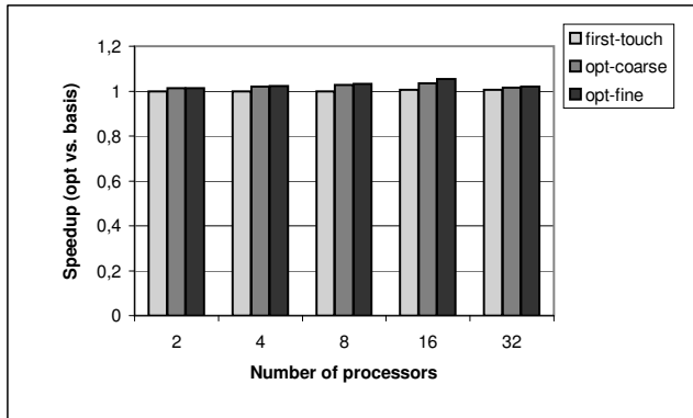
Figure 7. Improvement in execution time with the WATER application
