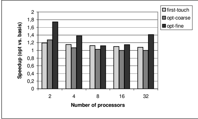
Figure 4. Improvement in execution time with the FFT application
